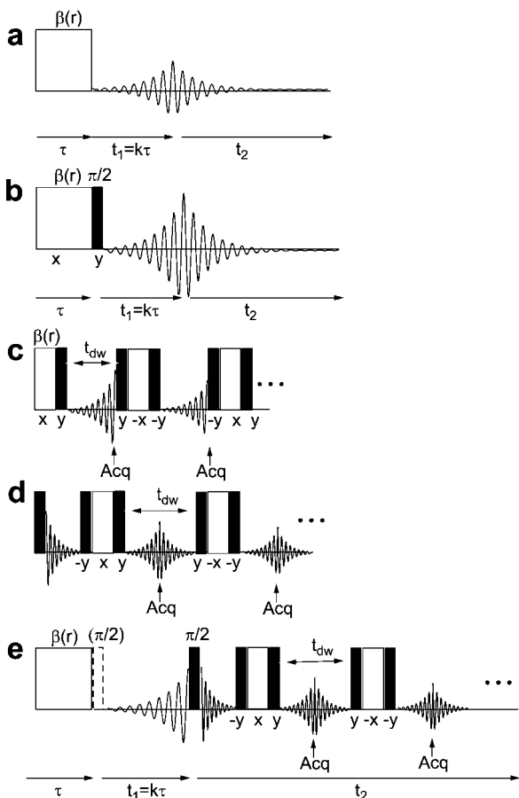
FIG. 1. Nutation echo based pulse sequences: ideal 90^\circ pulses (approximated by constant rotation composite pulses; see text) are depicted in black, and inhomogeneous RF pulses are depicted in white. (a) 2D nutation echo sequence in the absence of a 90^\circ pulse; (b) 2D nutation echo sequence with full signal recovery; (c) and (d) arrangements of inhomogeneous z -rotation composite pulses ( 90^\circ_{-y}[\beta(r)_x](90^\circ_y) ) for stroboscopic acquisition of resolved spectra; (e) COSY pulse sequence with refocusing B_1 gradient pulses in both dimensions. The 90^\circ pulse at the end of the inhomogeneous RF pulse in the indirect dimension is optional for signal enhancement.
